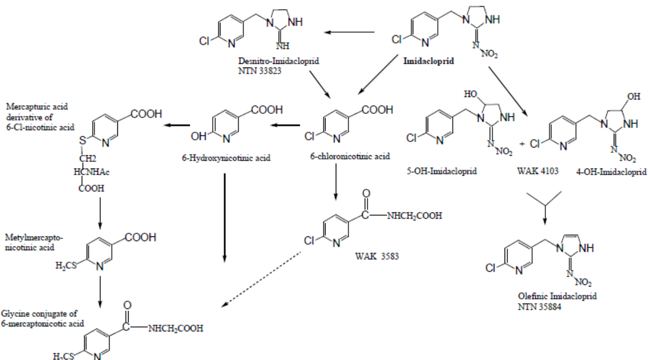
Figure 2: Proposed Metabolic Pathway for Imidacloprid
